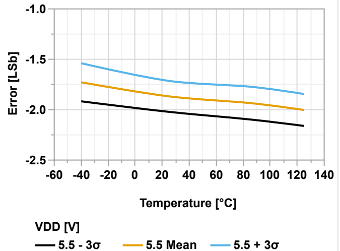
Figure 39-158. Offset Error vs. Temperature ( V_{\text{REFA}} = V_{\text{DD}} = 5.5\text{V} )
