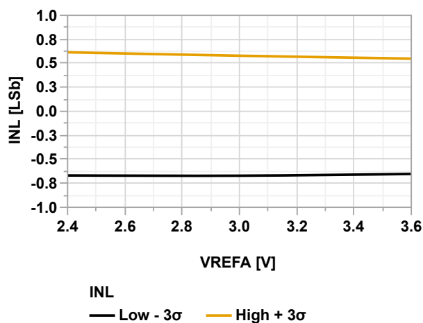
Figure 39-132. INL vs. V_{REFA} (ADC Differential Mode @60 kps, V_{DD} = 3.6V , T = 85^{\circ}C )
