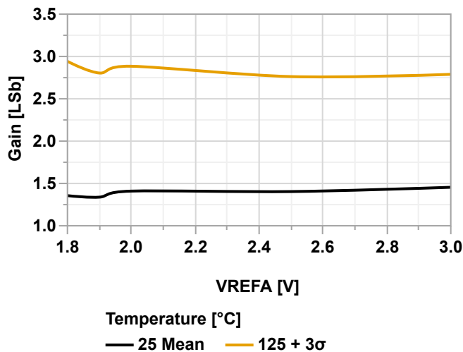
Figure 39-110. Gain Error vs. V_{REFA} (ADC Single Ended Mode @60 kps, V_{DD} = 3.0V )
