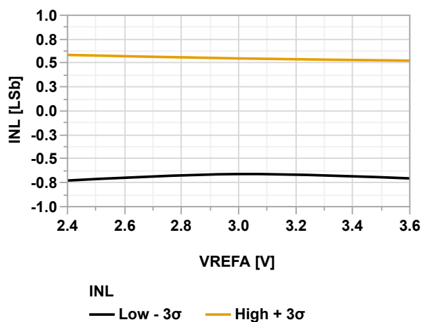
Figure 39-133. INL vs. V_{REFA} (ADC Differential Mode @60 kps, V_{DD} = 3.6V , T = 125^{\circ}C )
