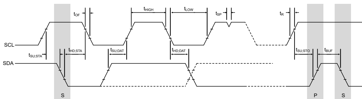
Figure 38-8. TWI - Timing Requirements
