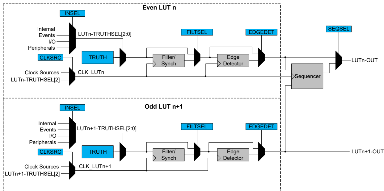
Figure 31-1. CCL Block Diagram
