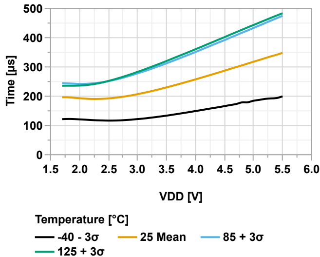
Figure 39-88. VREF Start-up Time vs. V_{DD}
