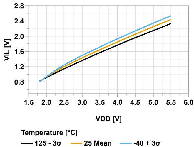
Figure 39-75. Input Pin with I 2 C Trigger - Maximum V_{IL} vs. V_{DD}
