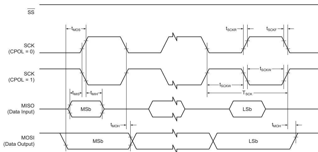
Figure 38-6. SPI - Timing Requirements in Host Mode
