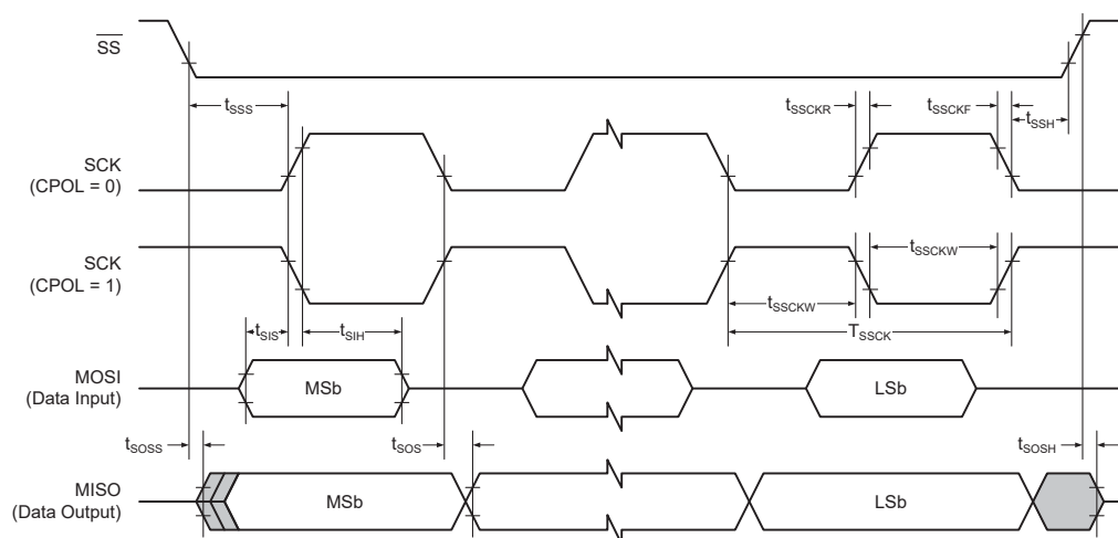
Figure 38-7. SPI - Timing Requirements in Client Mode
