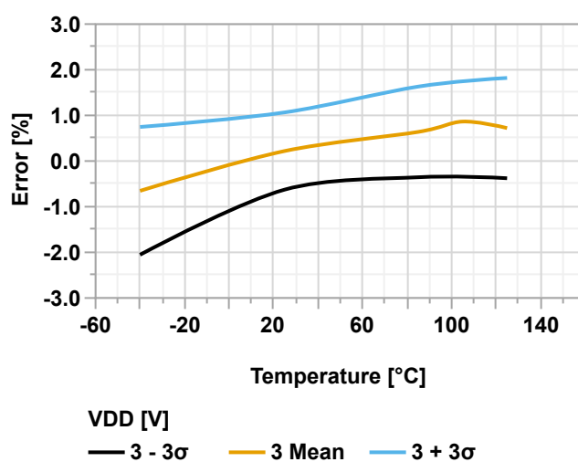
Figure 39-108. DACREF Voltage Error vs. Temperature ( V_{DD} = 3.0V , V_{VREF} = 2.5V )
