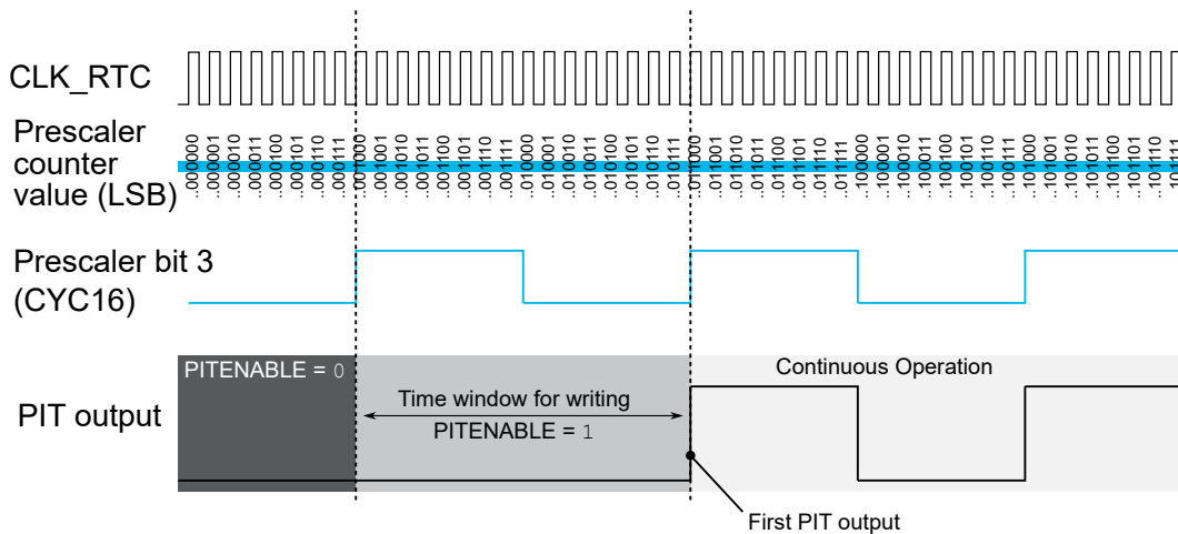
Figure 26-2. Timing Between PIT Enable and First Interrupt
