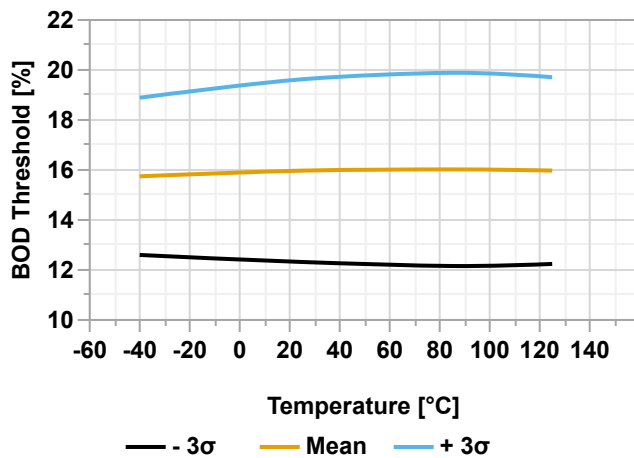
Figure 39-66. VLM Threshold vs. Temperature (VLMCTRL.VLMVLV = 0x02)
