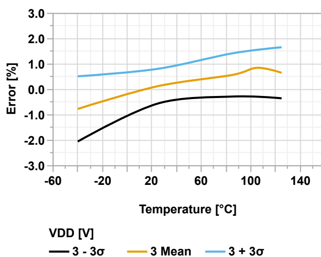
Figure 39-94. ADC0REF Voltage Error vs. Temperature ( V_{DD} = 3.0V , V_{VREF} = 2.5V )
