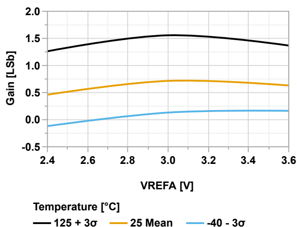
Figure 39-122. Negative Gain Error vs. V_{\text{REFA}} (ADC Differential Mode @60 kps, V_{\text{DD}} = 3.6\text{V} )
