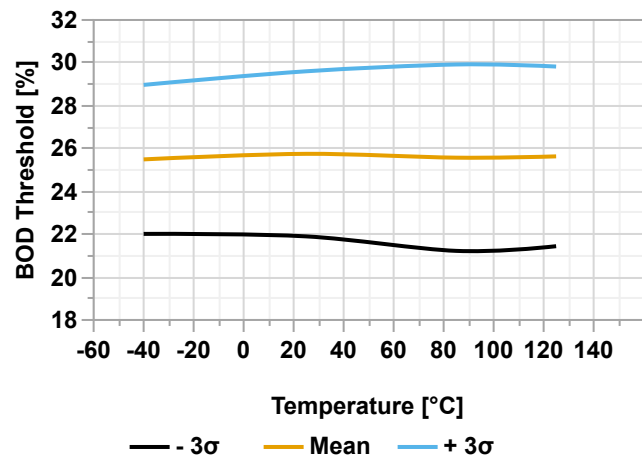
Figure 39-67. VLM Threshold vs. Temperature (VLMCTRL.VLMVLV = 0x03)
