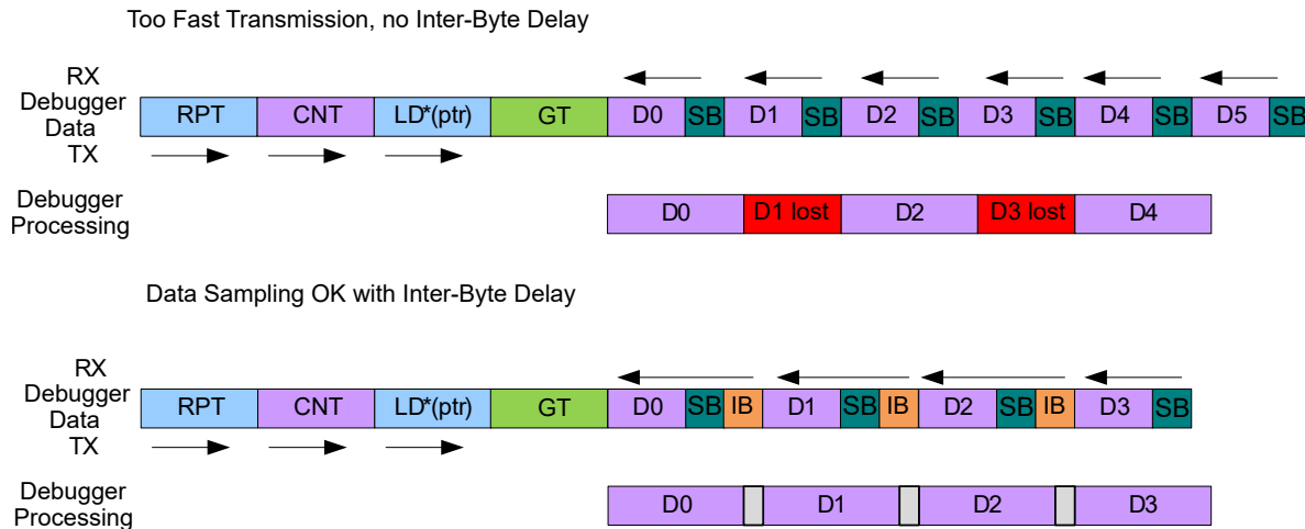
Figure 36-19. Inter-Byte Delay Example with LD and RPT
