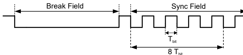
Figure 27-9. Auto-Baud Timing
