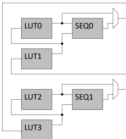
Figure 31-4. Linked LUT Input Selection
