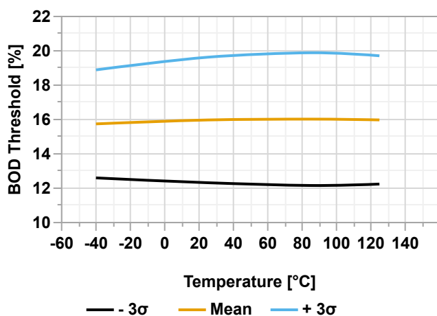
Figure 39-66. VLM Threshold vs. Temperature (VLMCTRL.VLMVL = 0x02)
