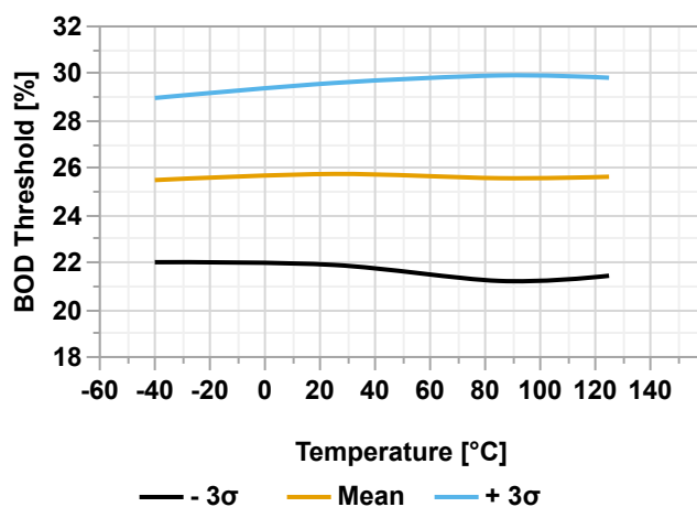
Figure 39-67. VLM Threshold vs. Temperature (VLMCTRL.VLMVL = 0x03)
