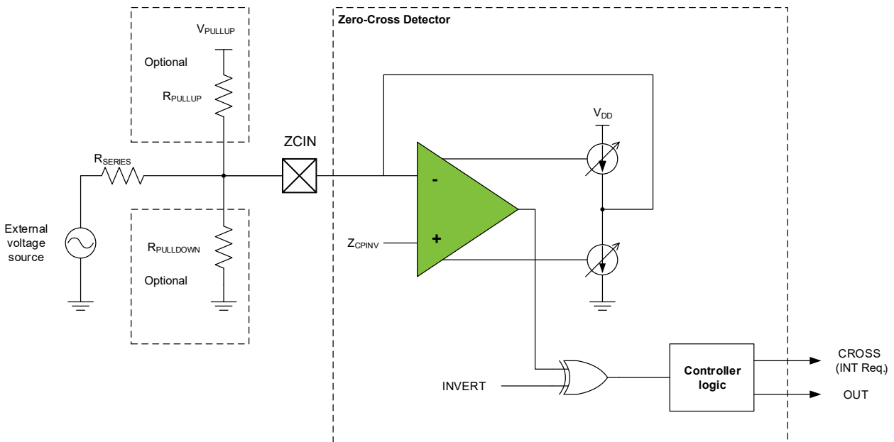
Figure 35-1. ZCD Block Diagram
