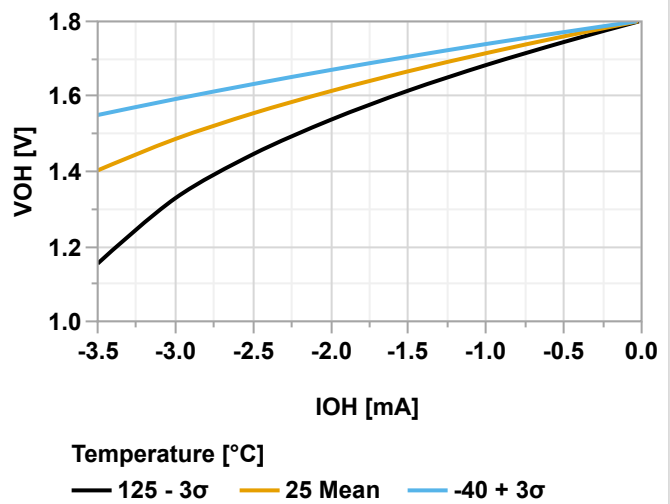
Figure 39-83. Output Pin - Minimum V_{OH} vs. Current, V_{DD} = 1.8 V
