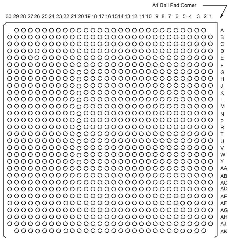
Figure 3-6. Package Bottom-View
