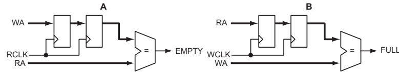
Figure 2-65. Overflow and Underflow Control
