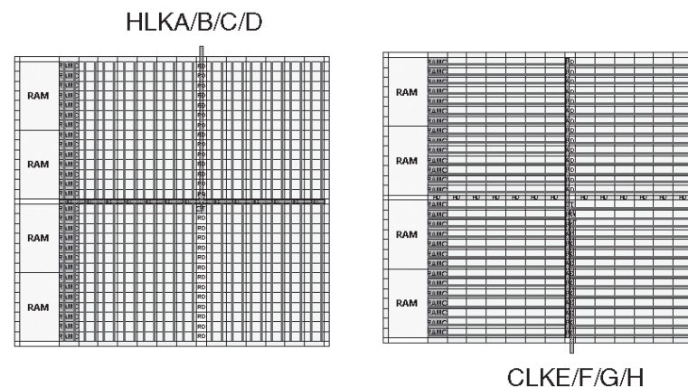
Figure 2-42. HCLK and CLK Distribution within a Core Tile
