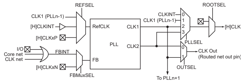
Figure 2-50. PLL Logical Interface
