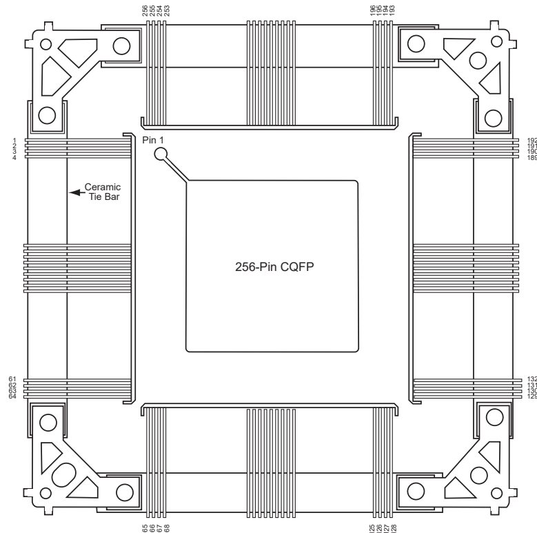
Figure 3-10. Package Bottom-View
