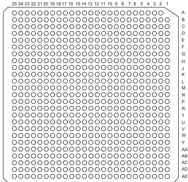
Figure 3-12. Package Bottom-View
