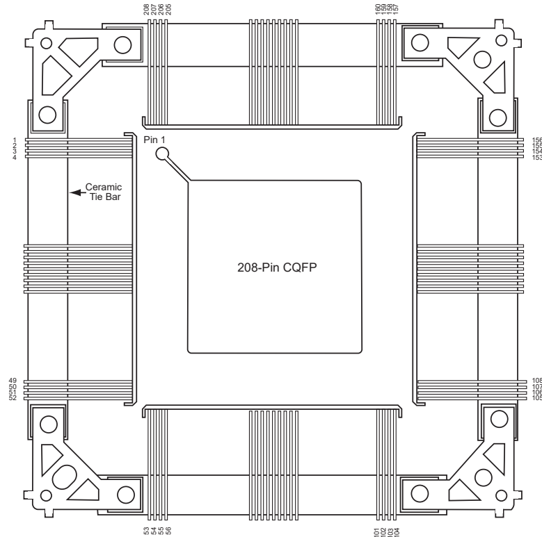
Figure 3-9. Package Bottom-View
