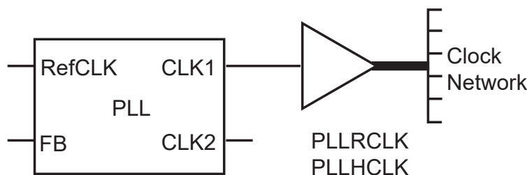
Figure 2-45. PLLRCLK and PLLHCLK
