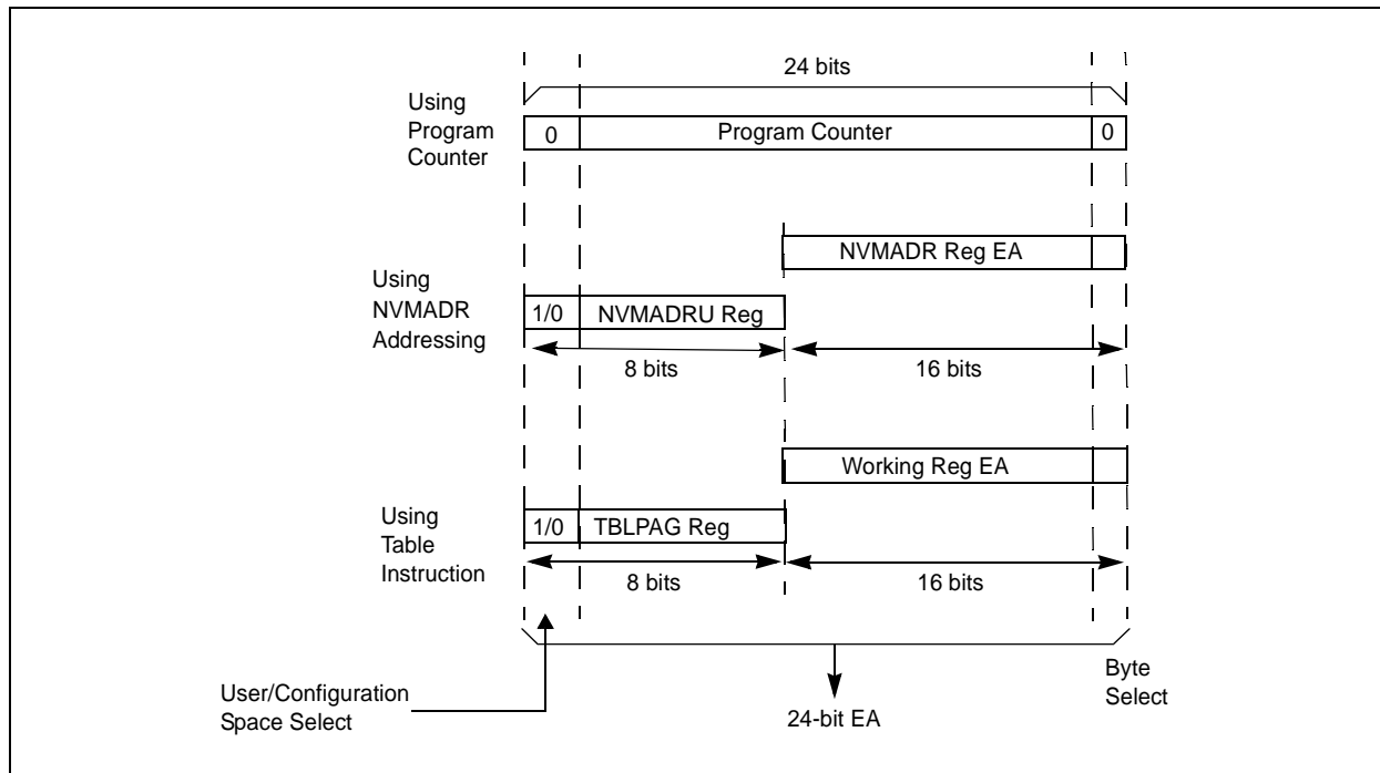
FIGURE 7-1: ADDRESSING FOR TABLE AND NVM REGISTERS
