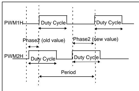
FIGURE 12-7: VARIABLE PHASE PWM
