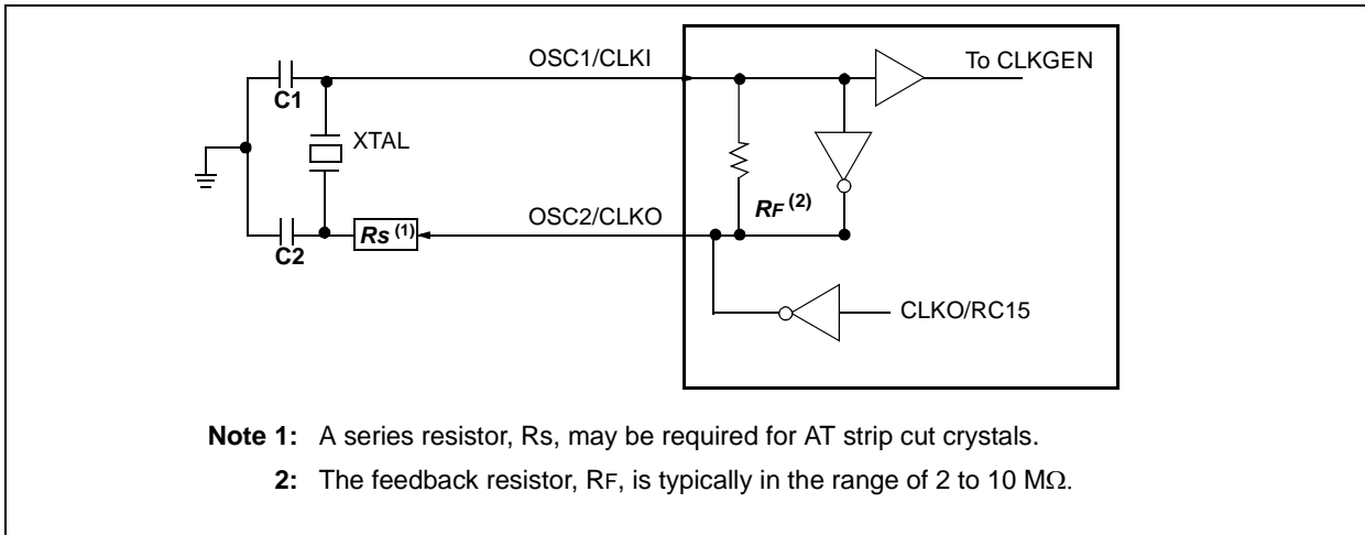
FIGURE 18-3: PRIMARY OSCILLATOR
