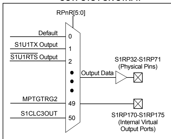
FIGURE 4-17: MULTIPLEXING REMAPPABLE OUTPUTS FOR S1RPn
