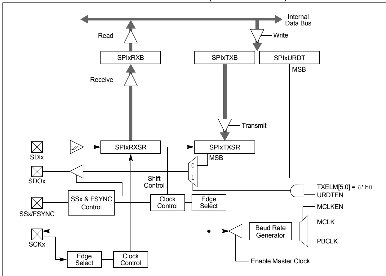
FIGURE 14-1: SPIx MODULE BLOCK DIAGRAM (STANDARD MODE)
