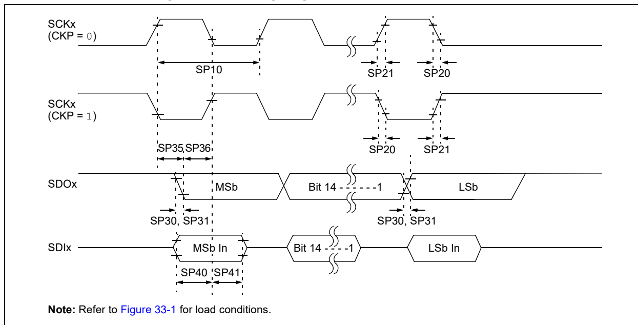
FIGURE 33-10: SPIx HOST MODE (FULL-DUPLEX, CKE = 0, CKP = x, SMP = 1) TIMING CHARACTERISTICS
