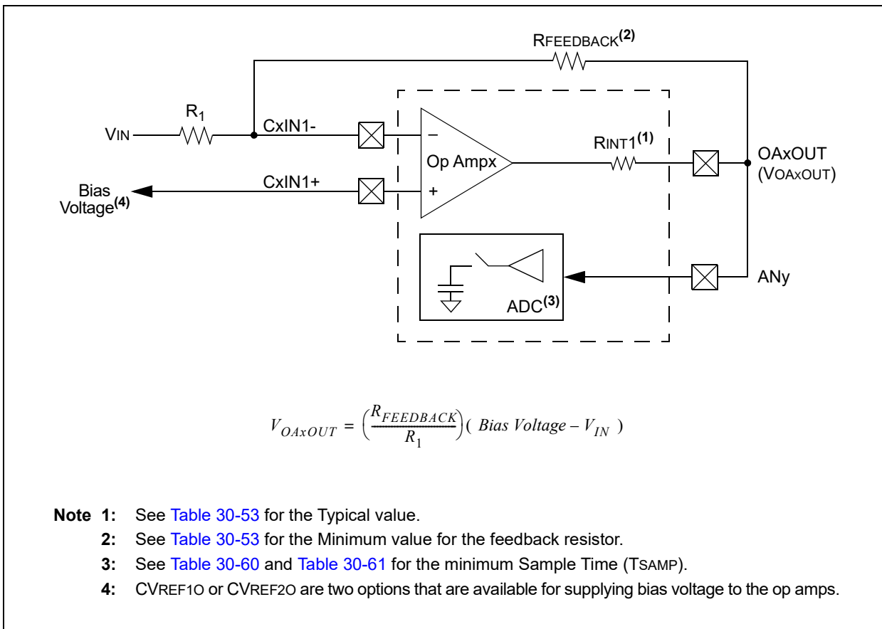
FIGURE 25-7: OP AMP CONFIGURATION B
