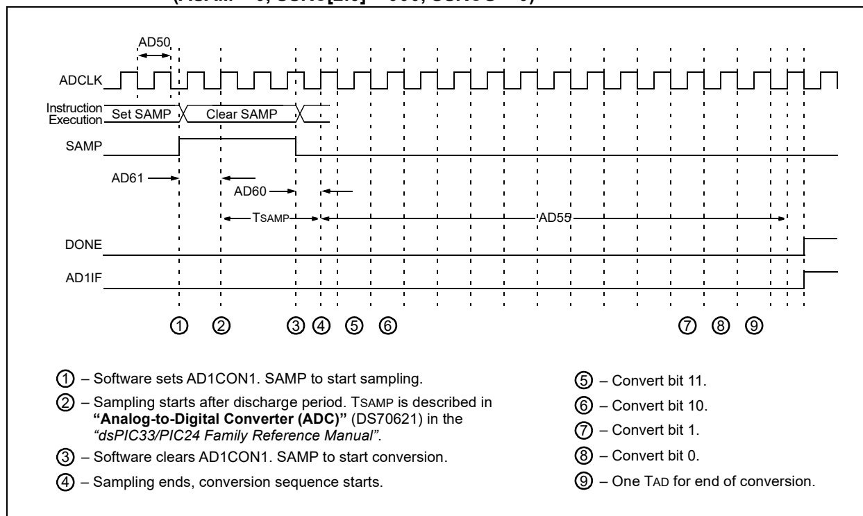
FIGURE 30-36: ADC CONVERSION (12-BIT MODE) TIMING CHARACTERISTICS (ASAM = 0, SSR[2:0] = 000, SSRG = 0)
