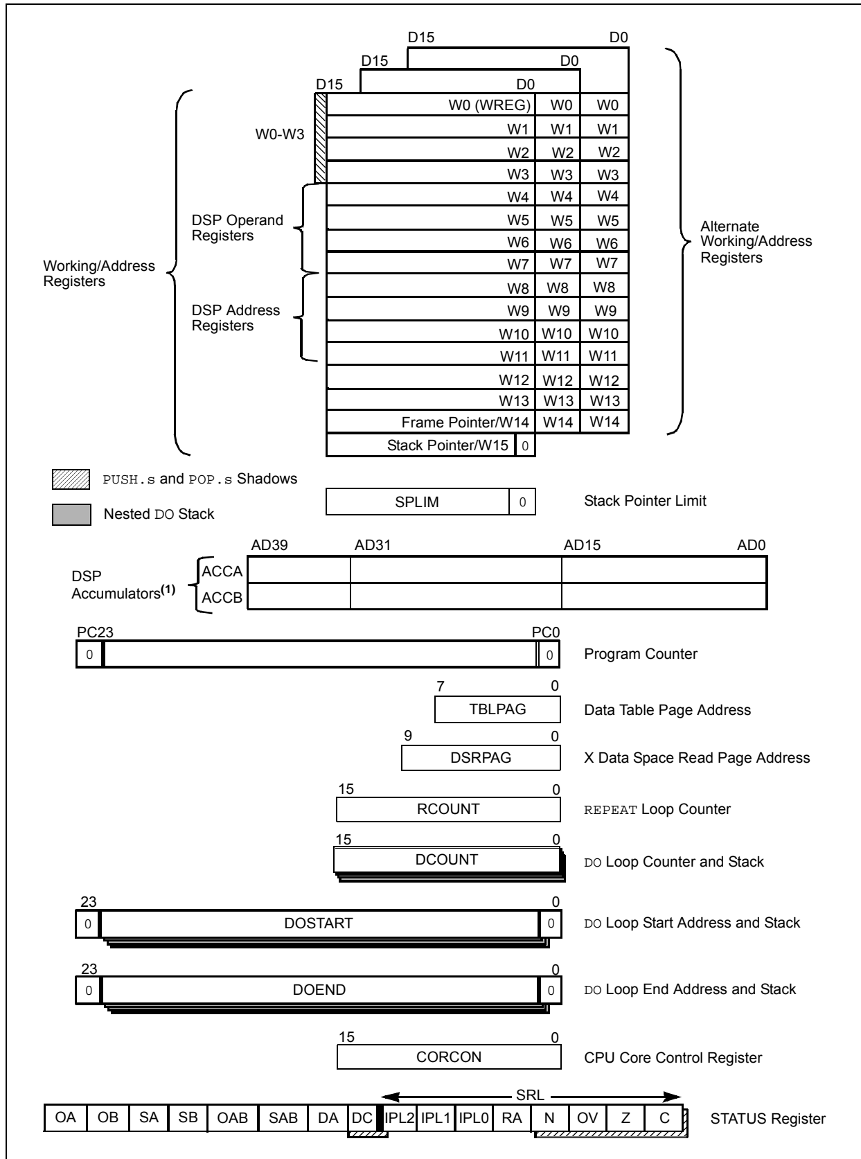
FIGURE 3-2: PROGRAMMER'S MODEL
