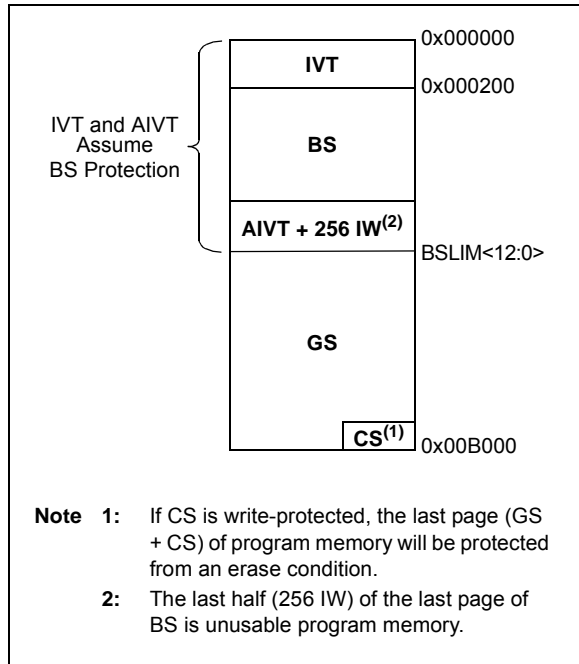
FIGURE 23-3: SECURITY SEGMENTS EXAMPLE FOR dsPIC33EP64GS50X DEVICES
