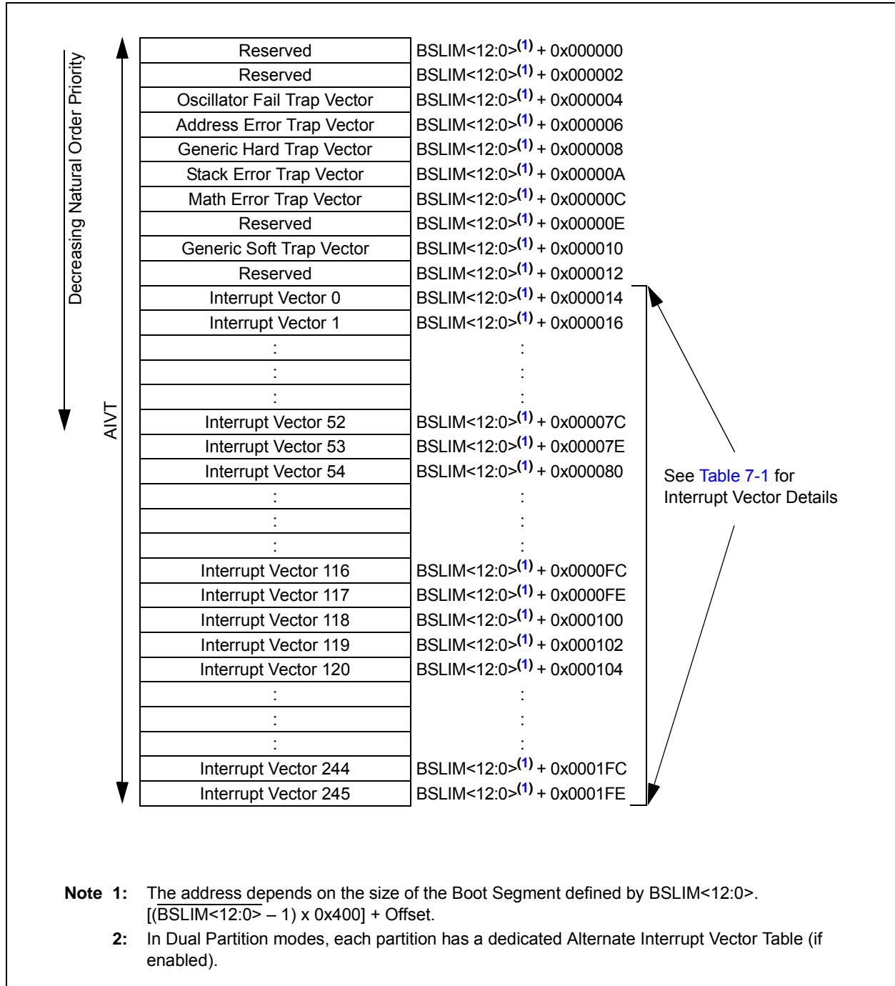
FIGURE 7-2: dsPIC33EPXXGS50X ALTERNATE INTERRUPT VECTOR TABLE (2)
