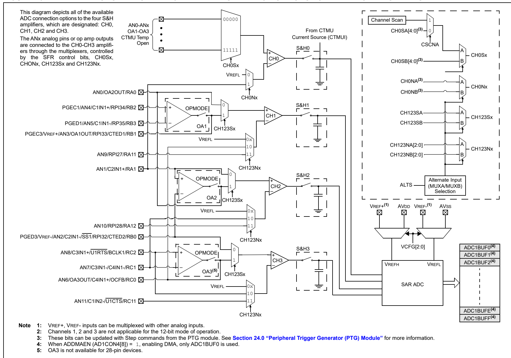
FIGURE 23-1: ADC MODULE BLOCK DIAGRAM WITH CONNECTION OPTIONS FOR ANx PINS AND OP AMPS
