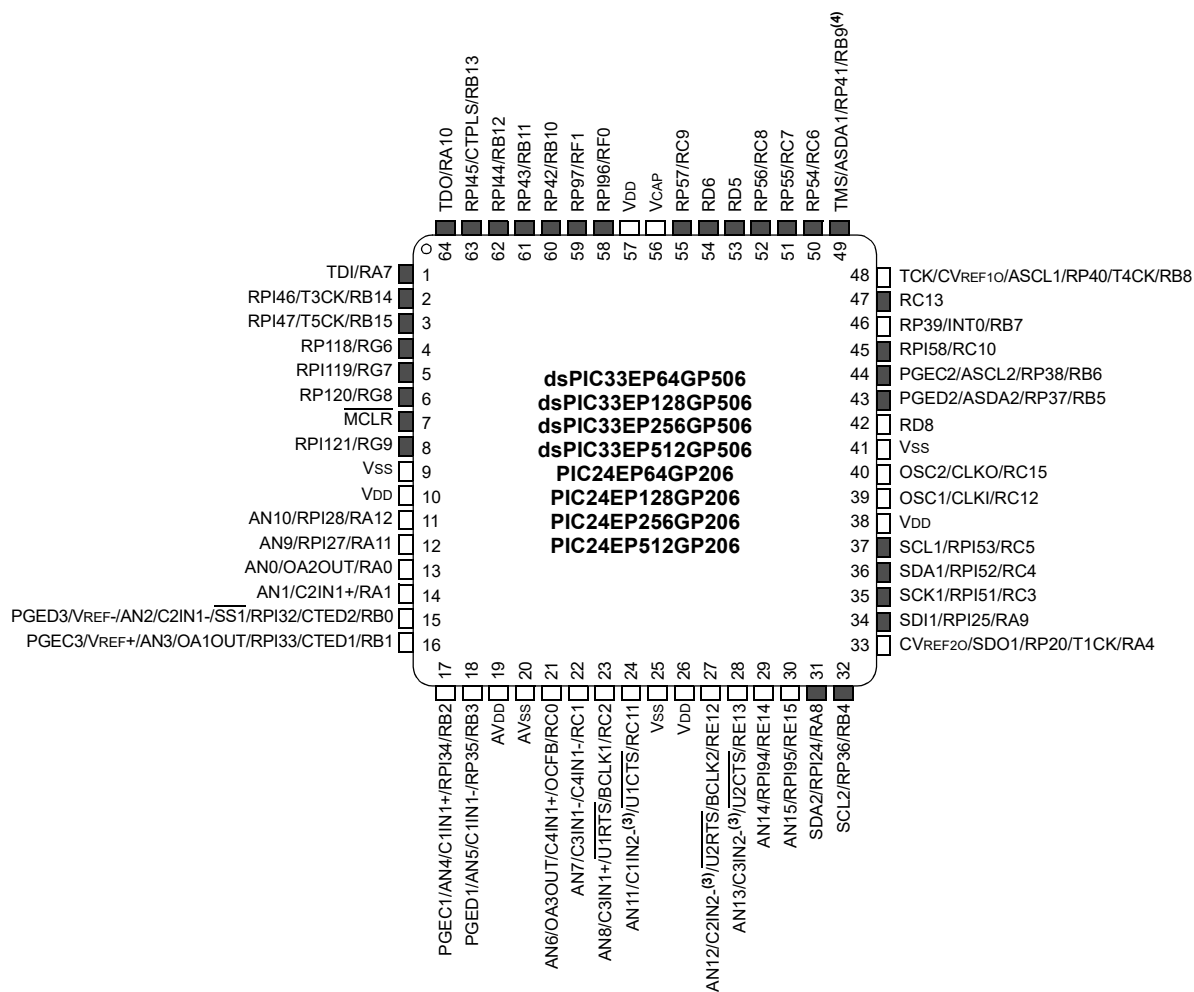
64-Pin TQFP (1,2,3)
