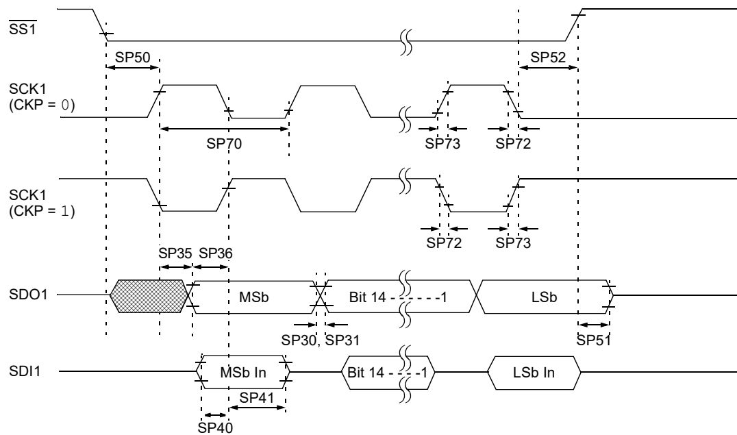
FIGURE 30-29: SPI1 SLAVE MODE (FULL-DUPLEX, CKE = 0, CKP = 0, SMP = 0) TIMING CHARACTERISTICS
