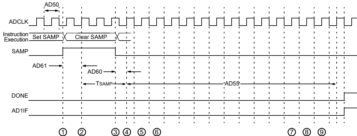
FIGURE 30-36: ADC CONVERSION (12-BIT MODE) TIMING CHARACTERISTICS (ASAM = 0, SSR[2:0] = 000, SSRG = 0)
