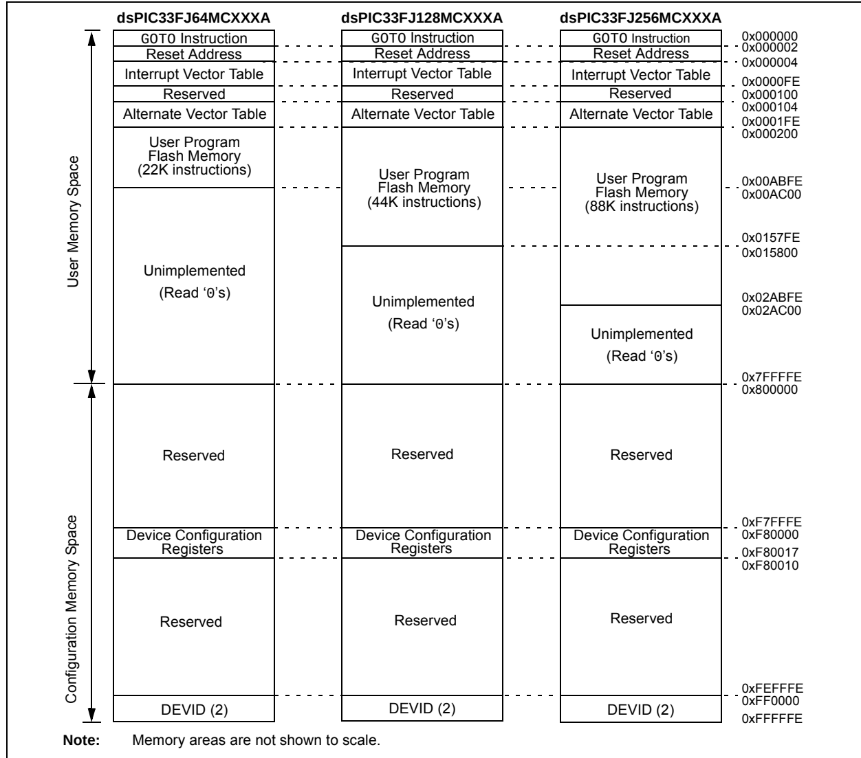
FIGURE 4-1: PROGRAM MEMORY MAP FOR dsPIC33FJXXMCMC06A/X08A/X10A DEVICES
