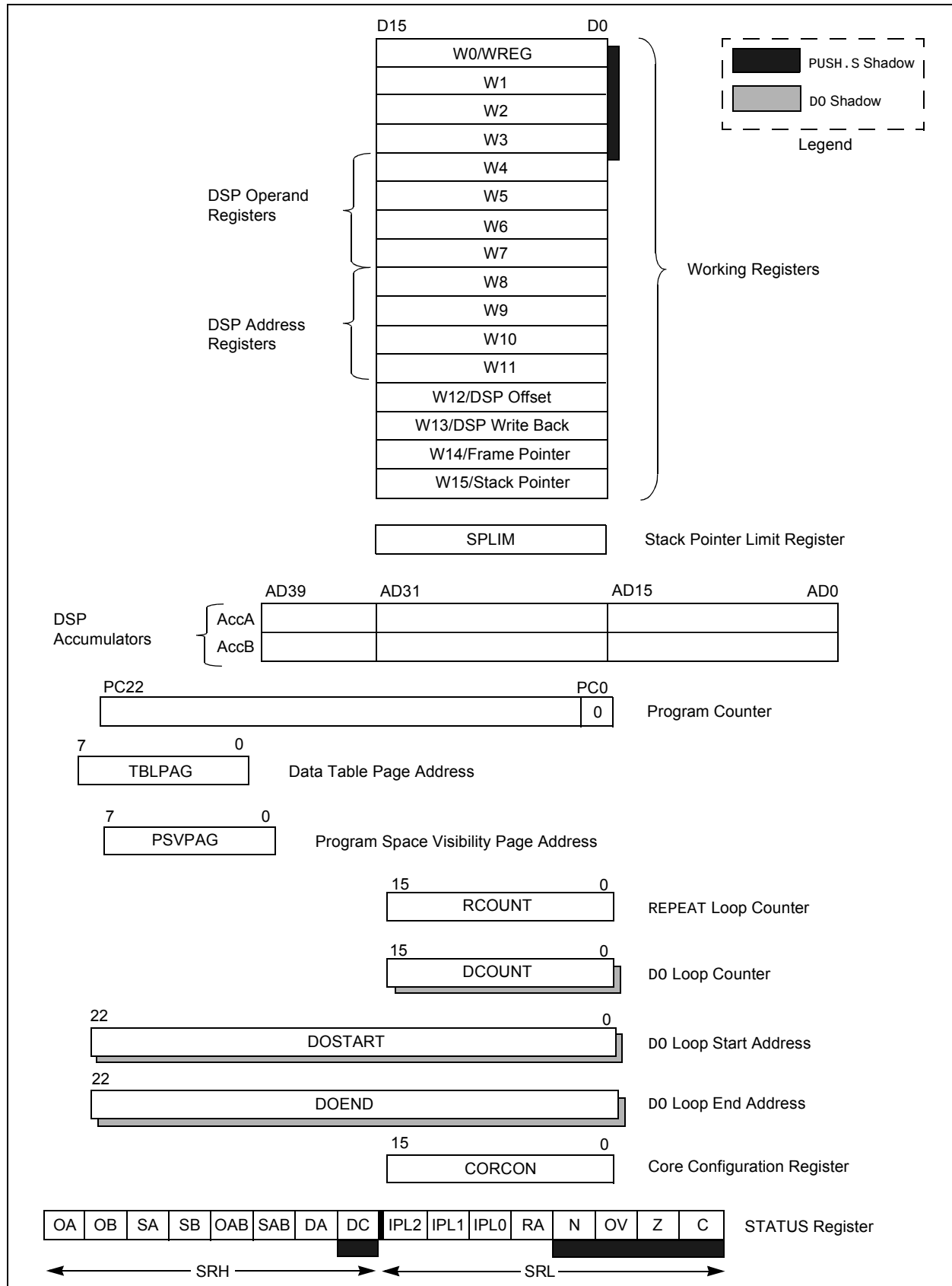
FIGURE 3-2: dsPIC33FJXXXMCX06A/X08A/X10A PROGRAMMER'S MODEL
