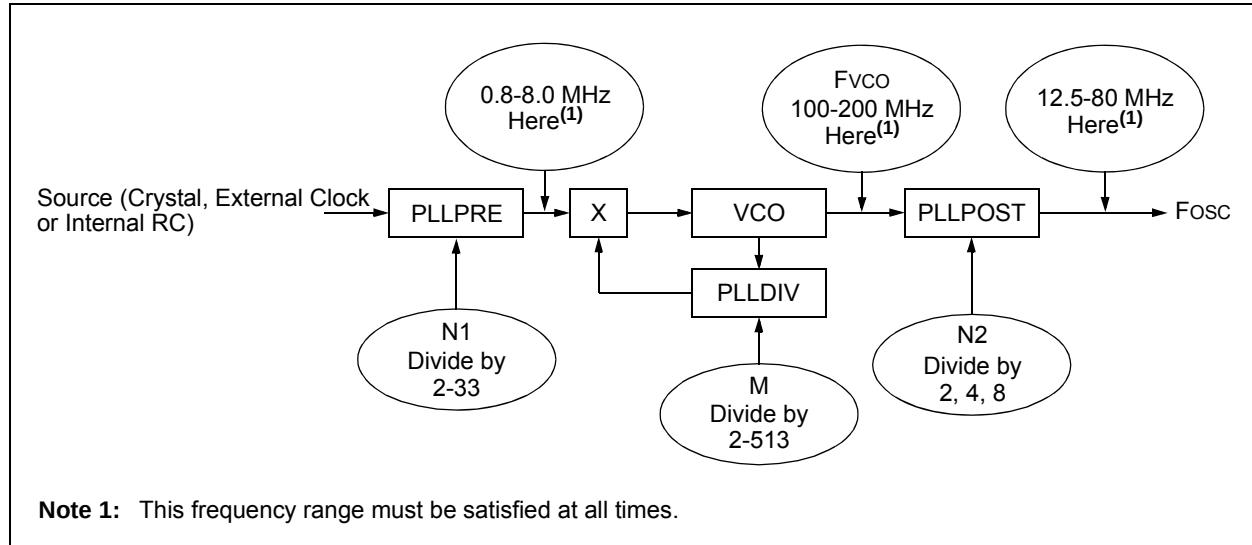
FIGURE 9-2: dsPIC33FJXXXMCX06A/X08A/X10A PLL BLOCK DIAGRAM
