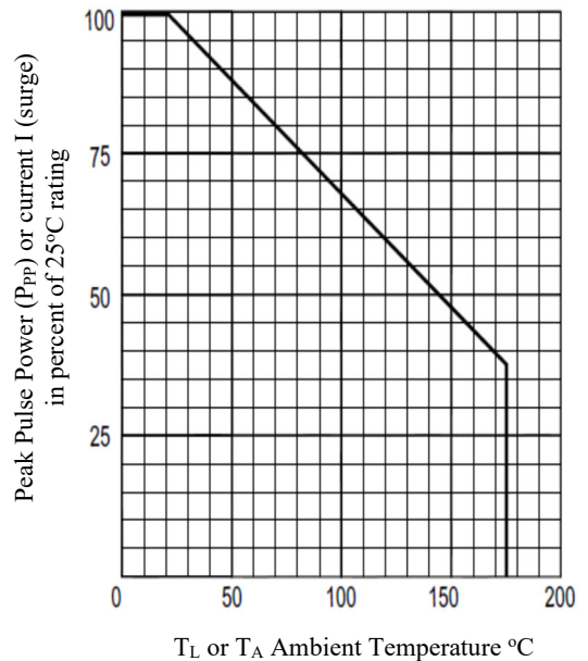
FIG. 4 Derating Curve
