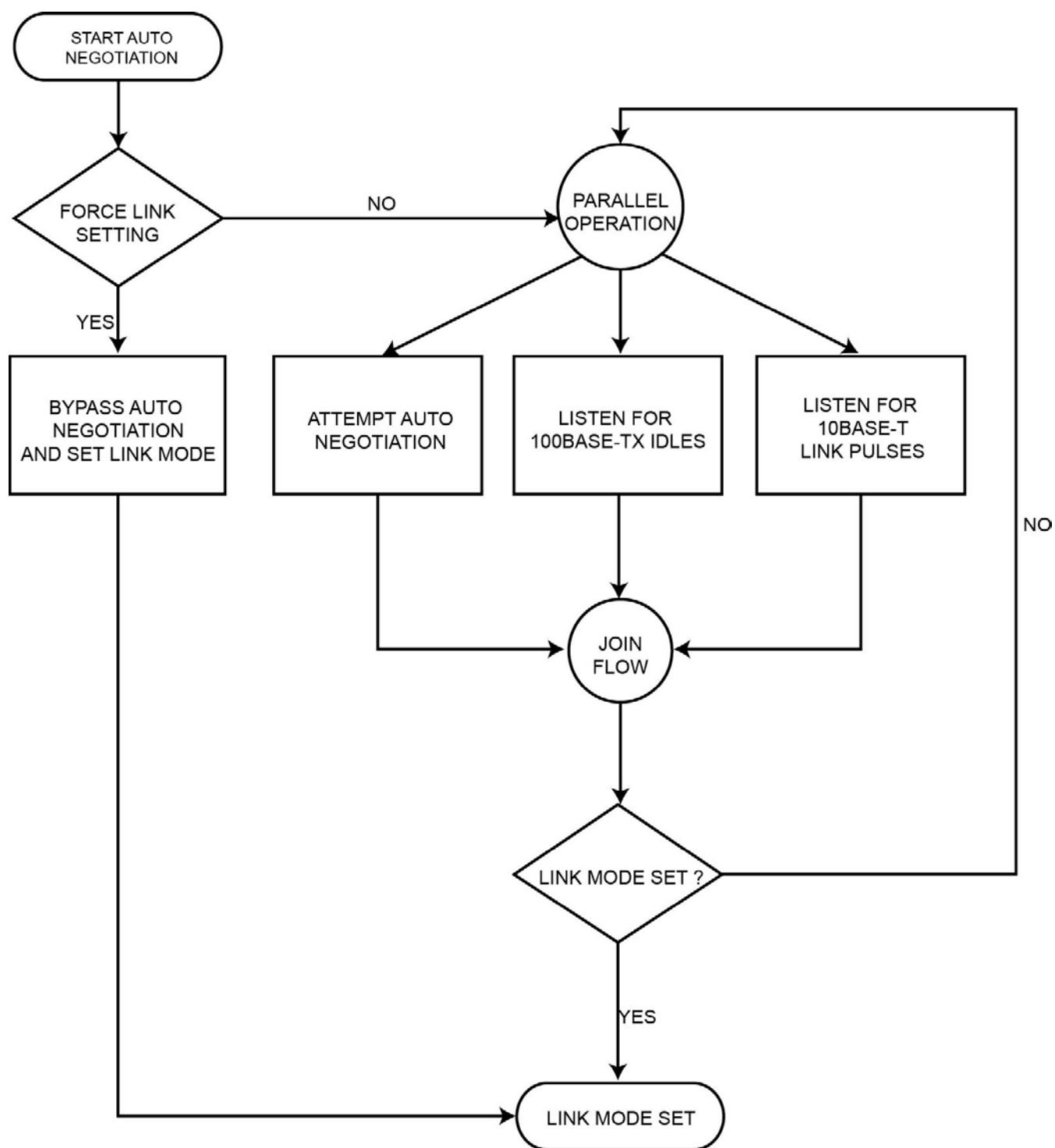
Figure 8. Auto-Negotiation
