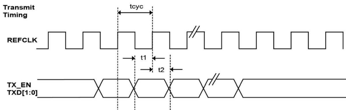
Figure 26. RMII Timing – Data Received from RMII
