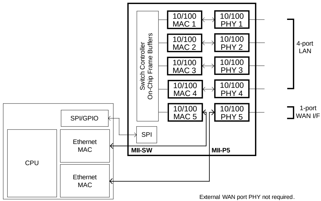
Figure 1. Broadband Gateway
