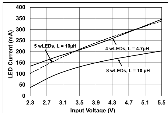
FIGURE 2-6: Maximum I_{LED} vs. V_{IN} .
