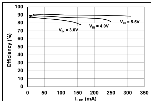
FIGURE 2-4: Four White LEDs, Efficiency vs. I_{LED} .
