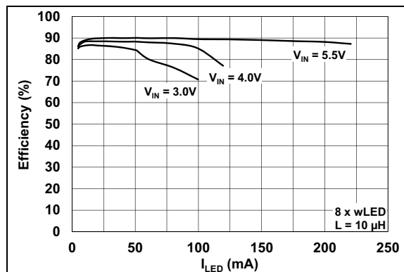
FIGURE 2-5: Eight White LEDs, Efficiency vs. I_{LED} .
