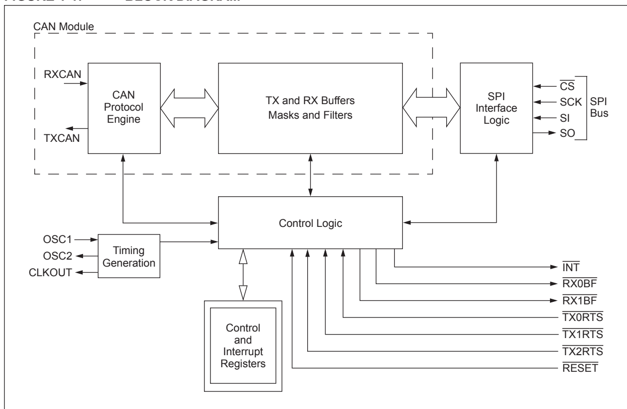
FIGURE 1-1: BLOCK DIAGRAM
