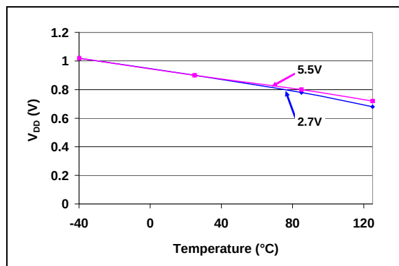
FIGURE 2-56: POR/BOR Trip point vs. V_{DD} and Temperature.
