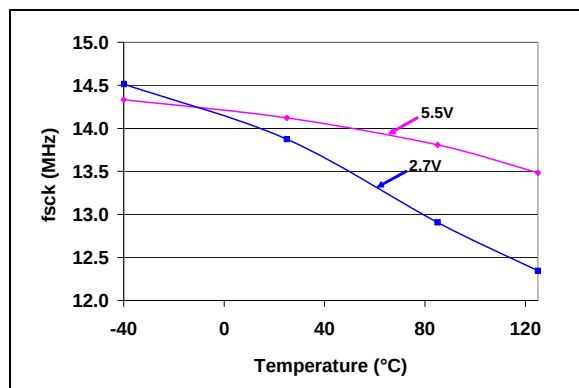
FIGURE 2-57: SCK Input Frequency vs. Voltage and Temperature.
