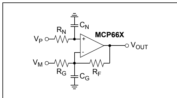
FIGURE 4-8: Amplifier with Parasitic Capacitance.
