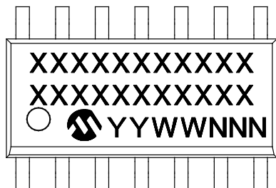
14-Lead SOIC (3.90 mm) (MCP660, MCP664)
