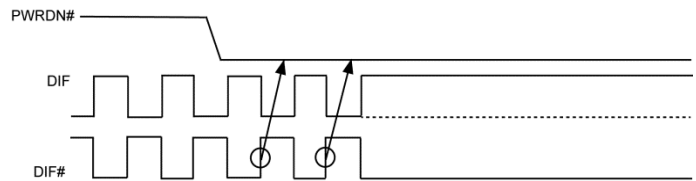
Figure 8. PWRDN# Assertion
