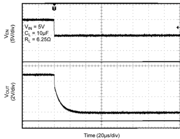
Enable Turn-Off Delay and Fall Time
