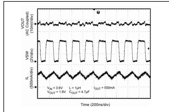
FIGURE 2-17: Switching Waveform.
