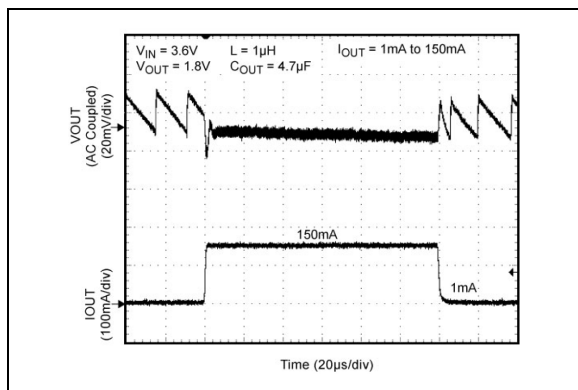
FIGURE 2-20: Load Transient.
