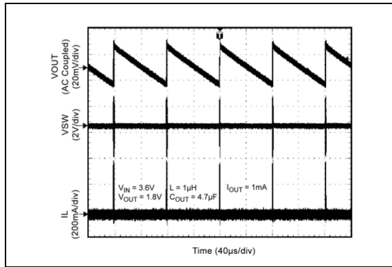
FIGURE 2-12: Switching Waveform.
