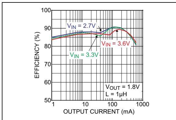
FIGURE 4-1: Efficiency V_{OUT} = 1.8V .
