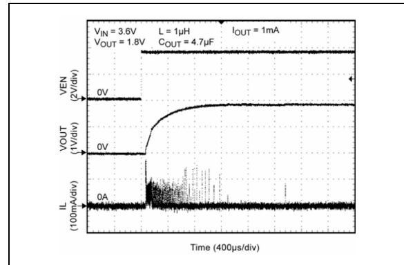
FIGURE 2-18: Start-Up Waveform.
