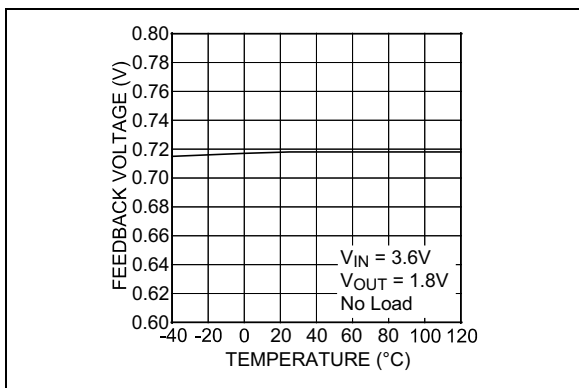
FIGURE 2-8: Feedback Voltage vs. Temperature.
