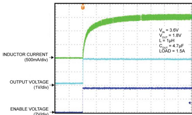
Start-Up Waveform
