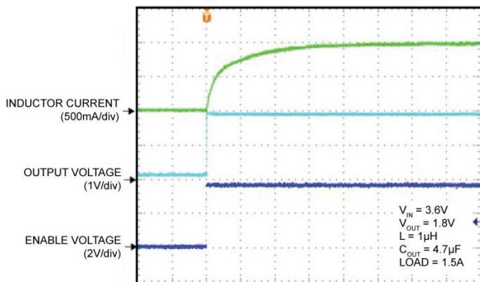
Start-Up Waveform
