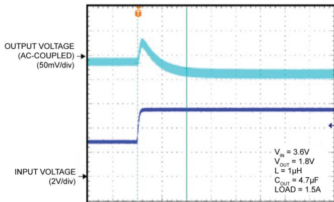
Line Transient 2.7V to 5.5V
