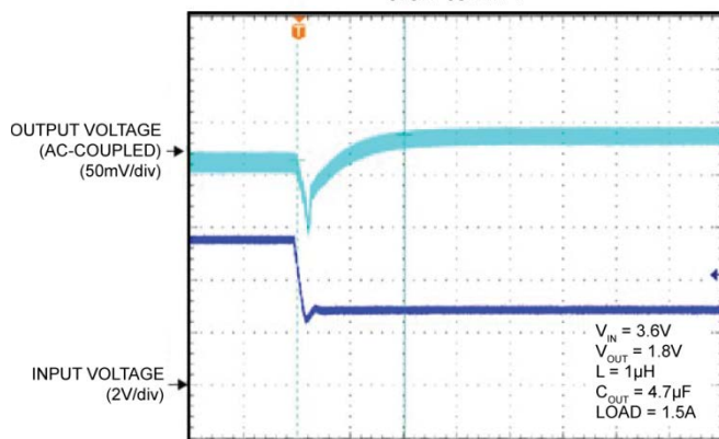
Line Transient 5.5V to 2.7V
