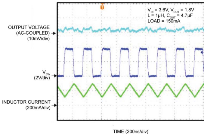
Switching Waveform Continuous Mode – 150mA
