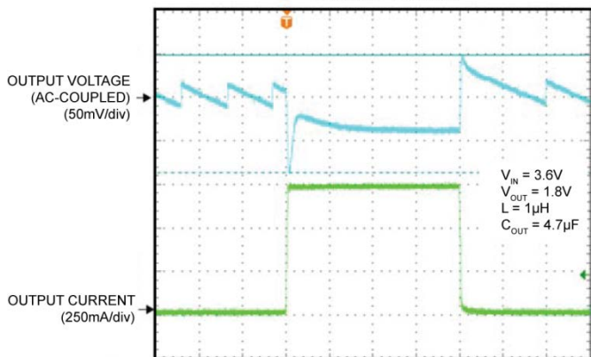
Load Transient 10mA to 750mA
