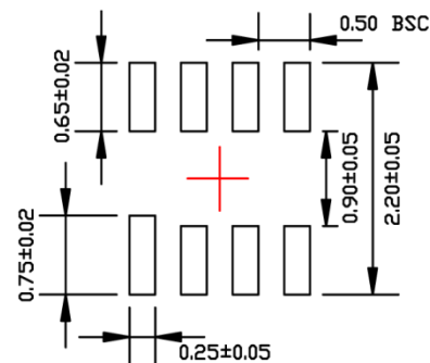
RECOMMENDED LANDING PATTERN
