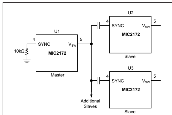
FIGURE 5-4: Master/Slave Synchronization.
