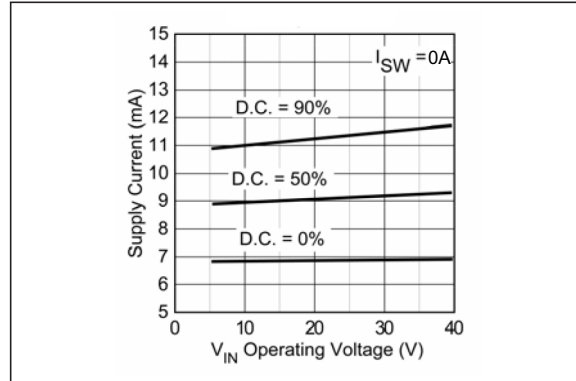
FIGURE 2-4: Supply Current vs. Operating Voltage.
