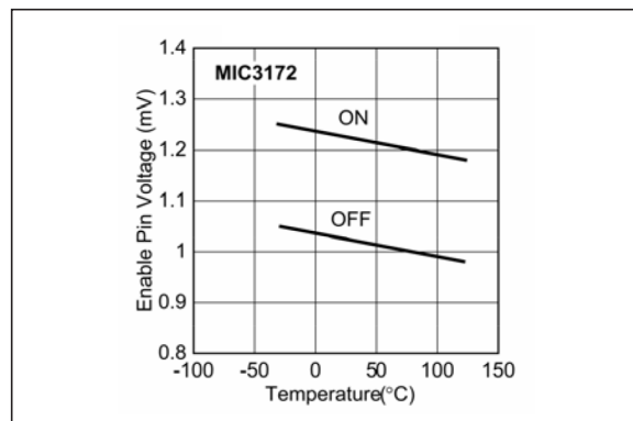
FIGURE 2-6: Enable Threshold Voltage vs. Temperature.
