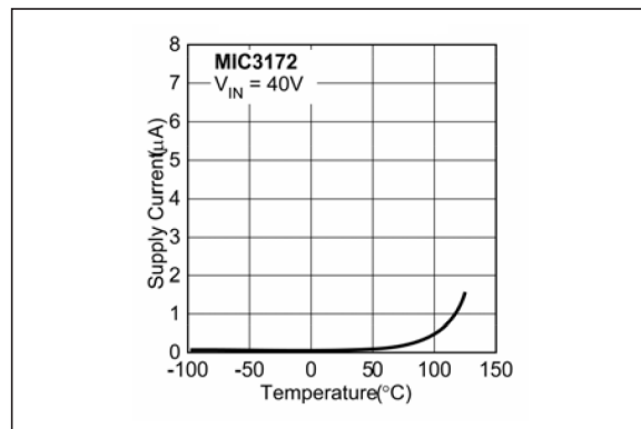
FIGURE 2-5: Supply Current (Shutdown Mode) vs. Temperature.
