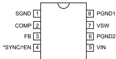
8-Pin DIP (N)
