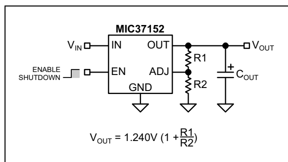
FIGURE 4-1: Adjustable Regulator with Resistors.
