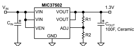
Adjustable Regulator
