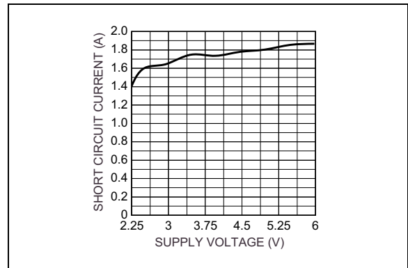
FIGURE 2-24: Short Circuit Current vs. Supply Voltage.
