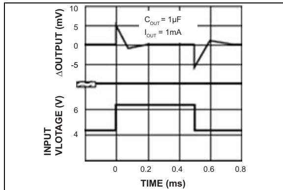
FIGURE 2-17: Line Transient.
