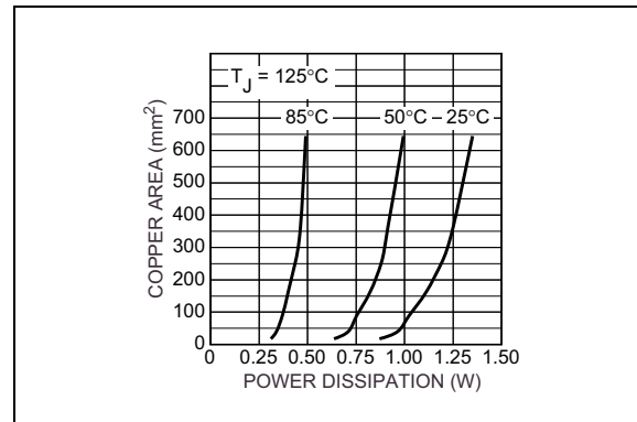
FIGURE 4-3: Copper Area vs. Power-SO Power Dissipation ( T_A ).
