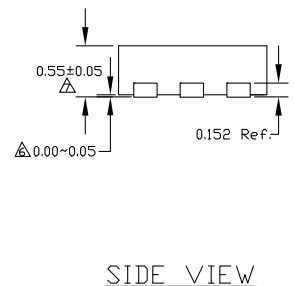
6-Pin 1.6mm x 1.6mm Thin MLF (MT)
