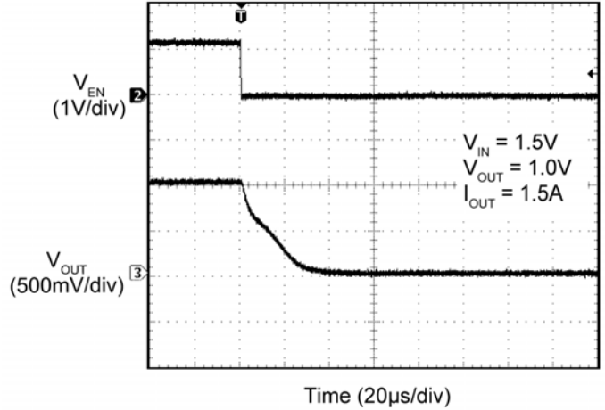
Enable Turn-Off
