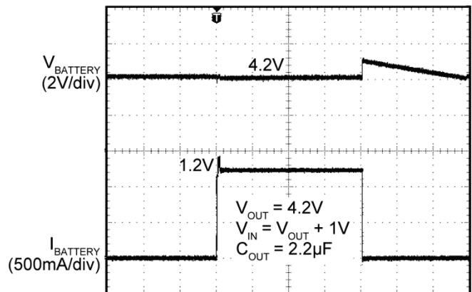
Time (1ms/div)
