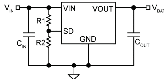
Figure 7. Auto-Shutdown using Shutdown Pin
