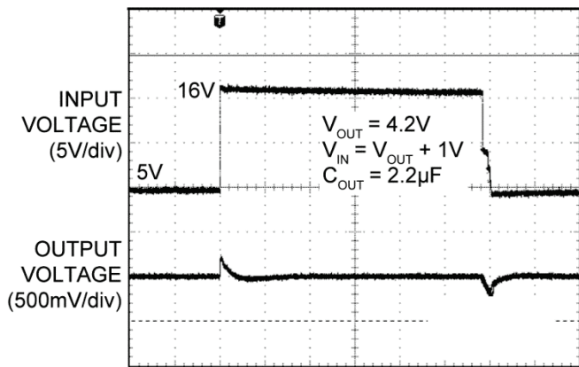
Line Transient
