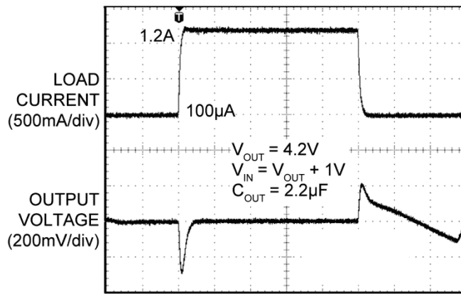
Load Transient
