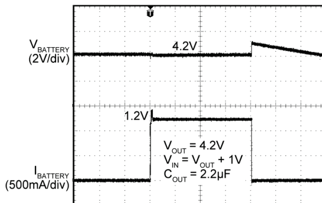
Battery Current Enable Transient
