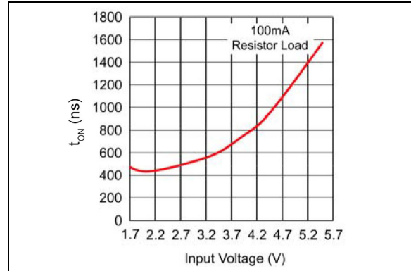
FIGURE 2-10: MIC94082/3 t_{ON} Delay vs. Input Voltage.
