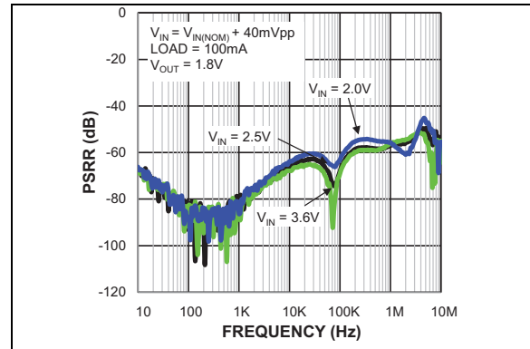
FIGURE 2-4: PSRR C_{OUT} = 1 \mu\text{F} .
