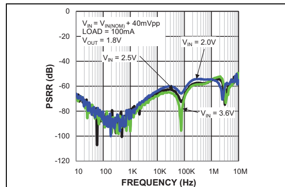
FIGURE 2-6: PSRR C_{OUT} = 2.2 \mu\text{F} .
