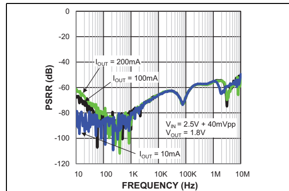
FIGURE 2-5: PSRR C_{OUT} = 2.2 \mu\text{F} .
