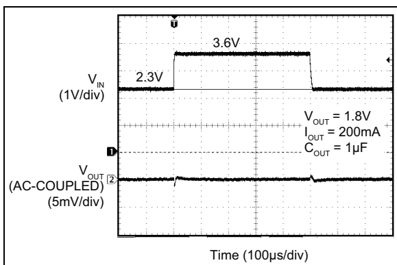
FIGURE 2-20: Line Transient (2.6V to 3.6V).
