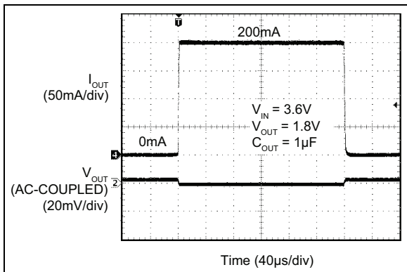
FIGURE 2-19: Load Transient (0 mA to 200 mA).
