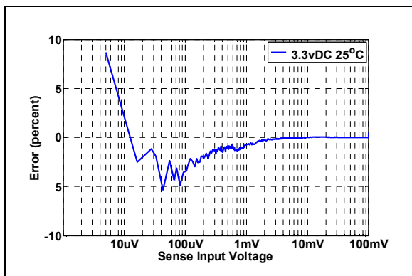
FIGURE 2-1: V_{SENSE} Error vs. V_{SENSE} Input Voltage.
