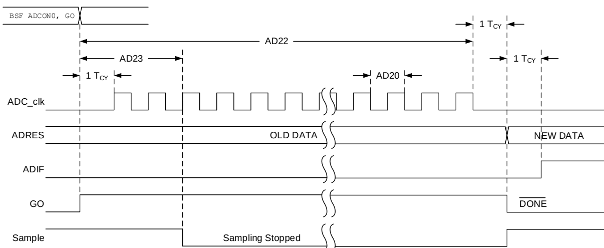
Figure 32-9. ADC Conversion Timing (ADC Clock F_{OSC} -Based)
