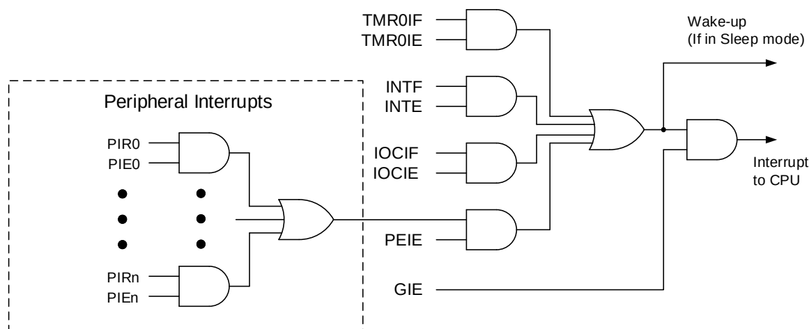
Figure 12-1. Interrupt Logic
