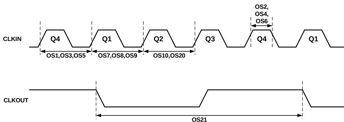
Figure 32-4. Clock Timing
