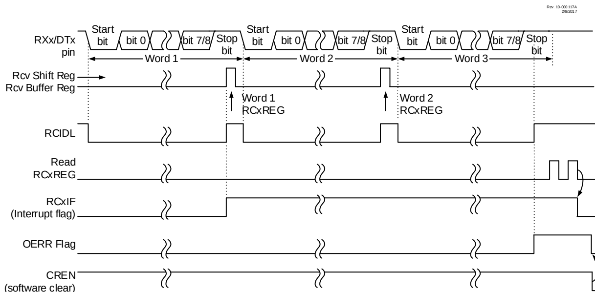
Figure 24-5. Asynchronous Reception
