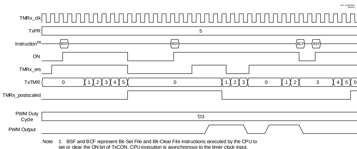
Figure 21-12. Level Triggered Hardware Limit One Shot Mode Timing Diagram (MODE = 'b10110)
