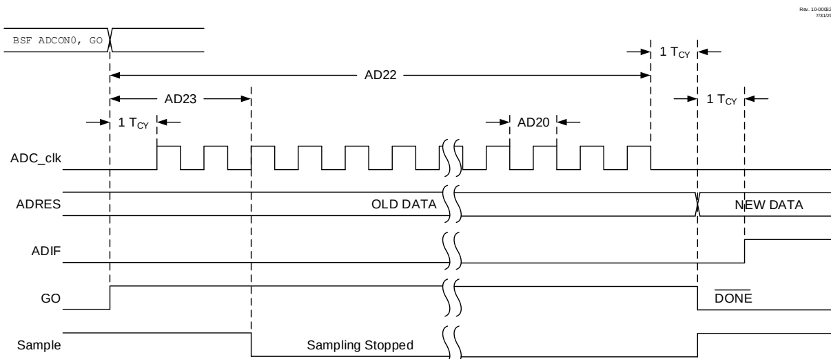
Figure 32-9. ADC Conversion Timing (ADC Clock F_{OSC} -Based)
