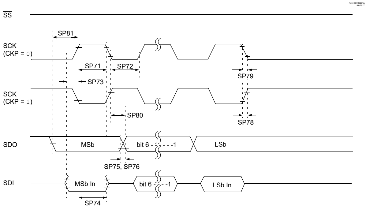
Figure 32-16. SPI Host Mode Timing (CKE = 1, SMP = 1)
