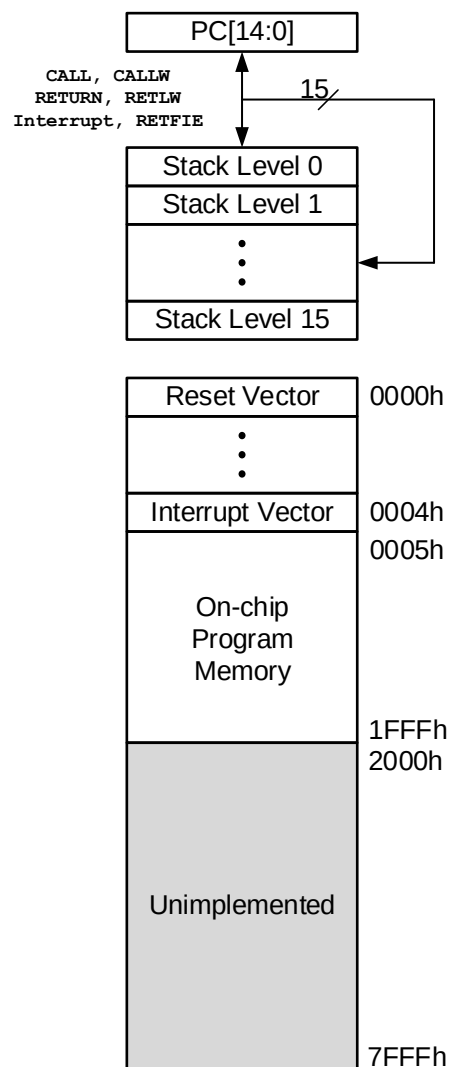
Figure 9-2. Program Memory and Stack (PIC16F15275)
