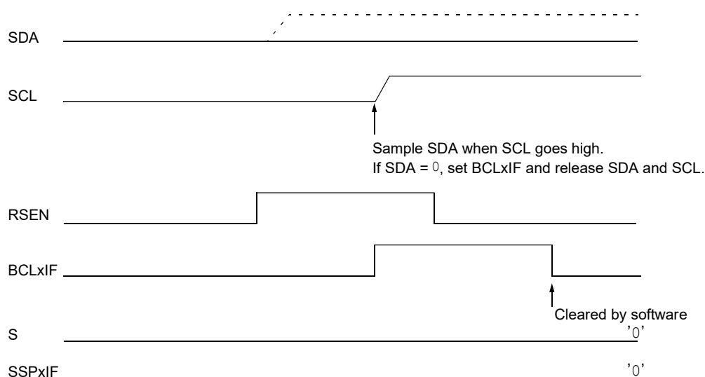
Figure 25-38. Bus Collision During a Repeated Start Condition (Case 1)
