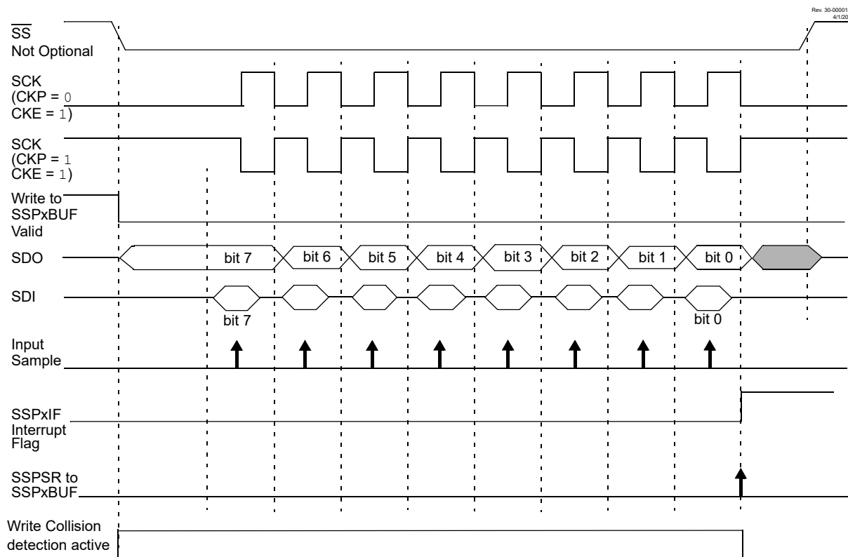
Figure 25-8. SPI Mode Waveform (Client Mode with CKE = 1)
